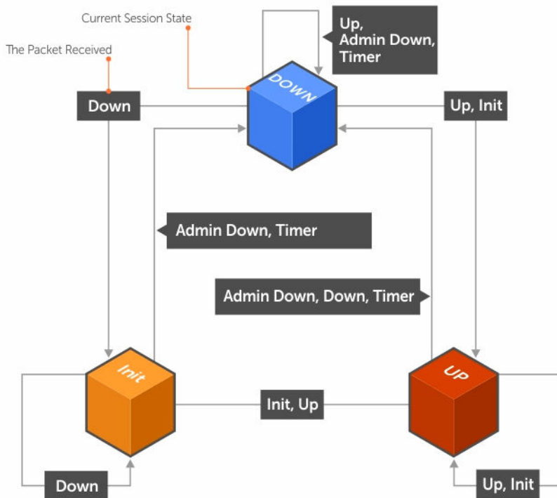
Figure 11. Session State Changes
