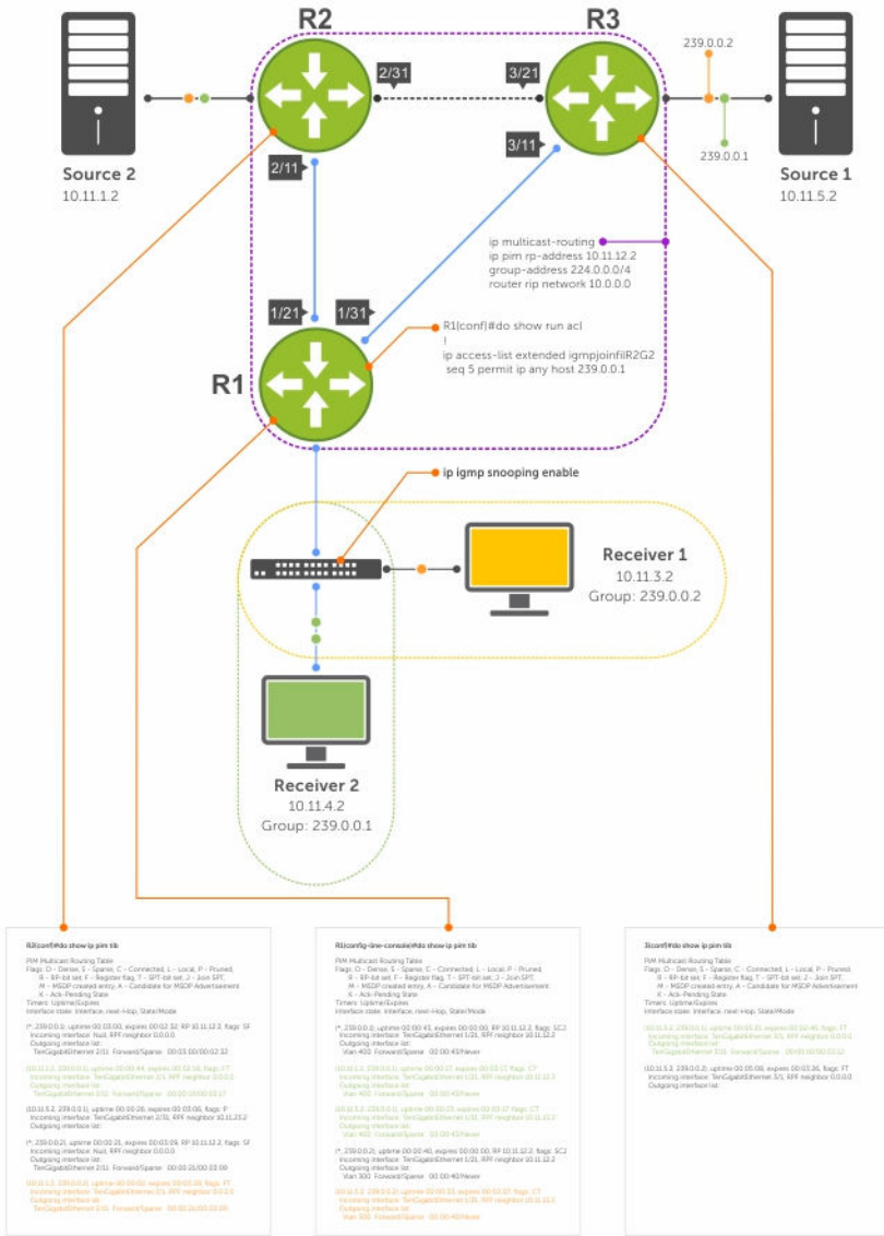
Figure 94. Preventing a Source from Transmitting to a Group
