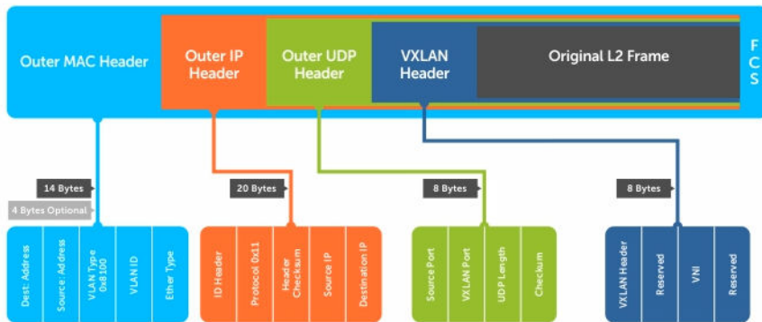
Figure 142. VXLAN Frame Format
