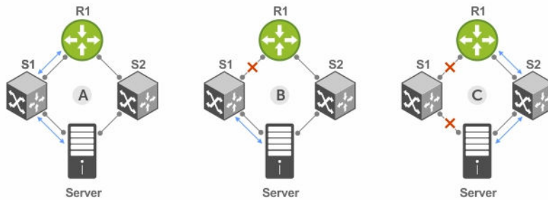
Figure 131. Uplink Failure Detection Example
