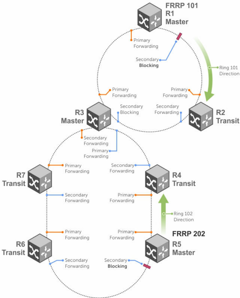
Figure 41. Example of Multiple Rings Connected by Single Switch
