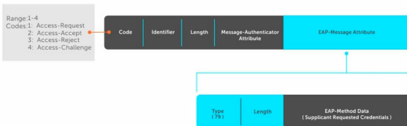
Figure 6. EAP Over RADIUS
