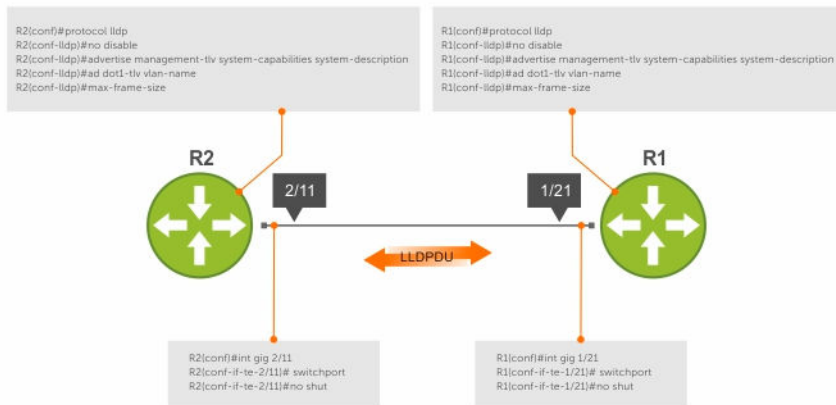
Figure 79. Configuring LLDP
