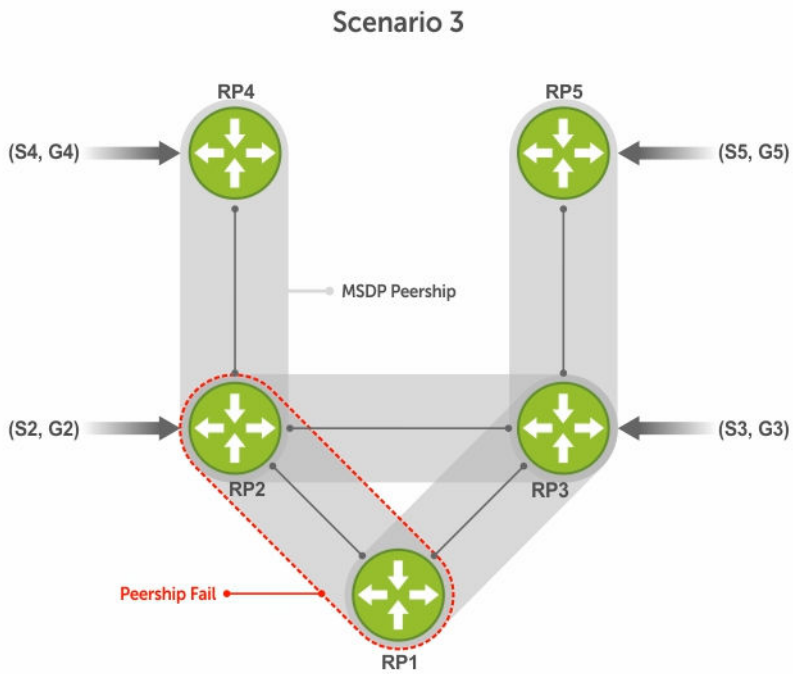
Figure 88. MSDP Default Peer, Scenario 3
