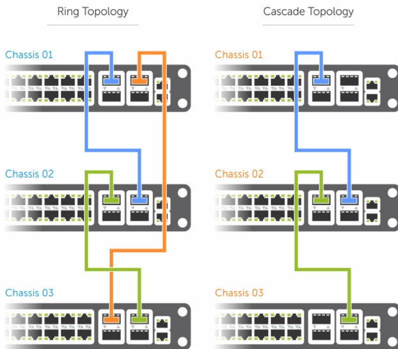
Figure 120. Supported Stacking Topologies
