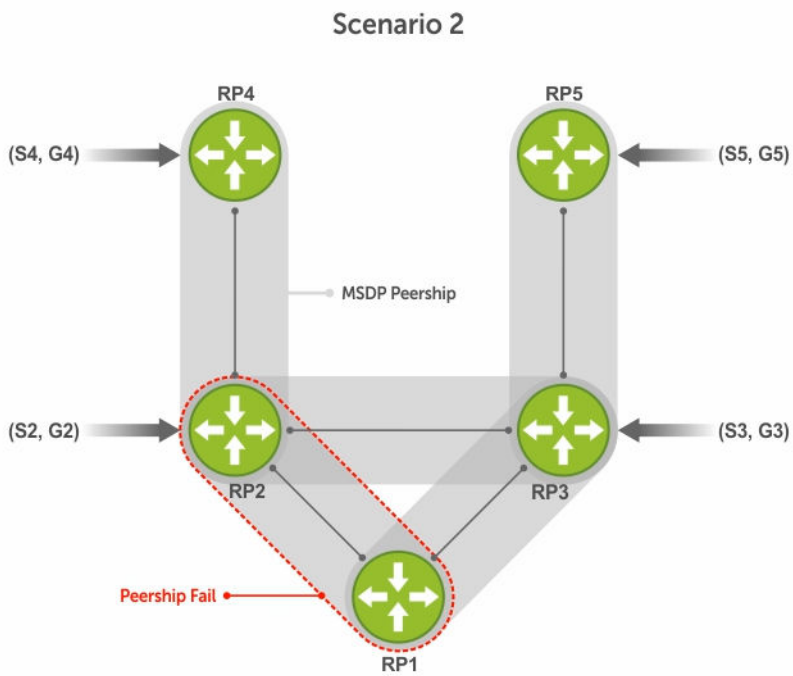
Figure 87. MSDP Default Peer, Scenario 2
