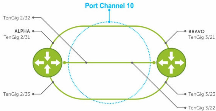
Figure 62. LACP Basic Configuration Example
