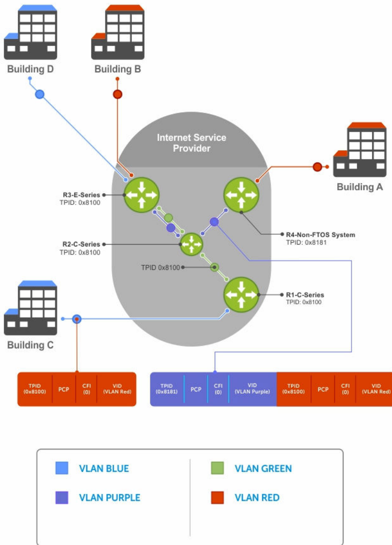
Figure 114. Single and Double-Tag TPID Match
