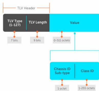
Figure 73. Type, Length, Value (TLV) Segment
