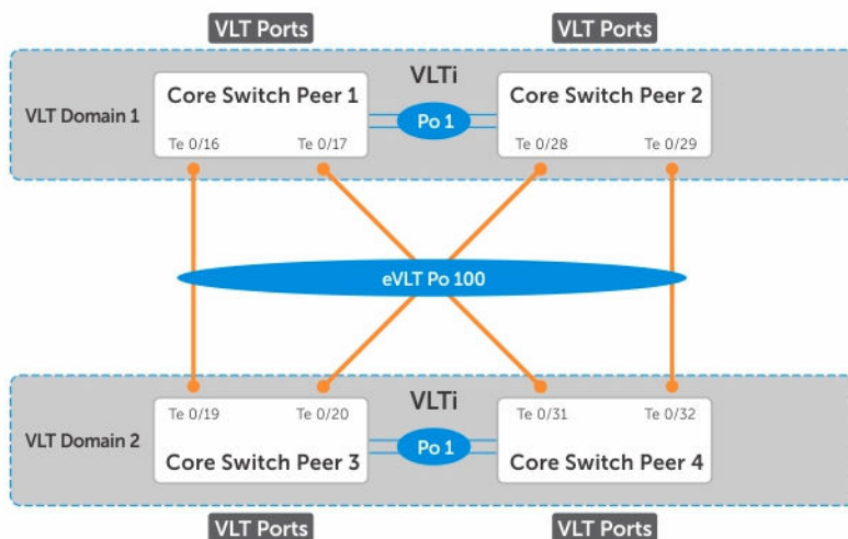
Figure 138. eVLT Configuration Example
