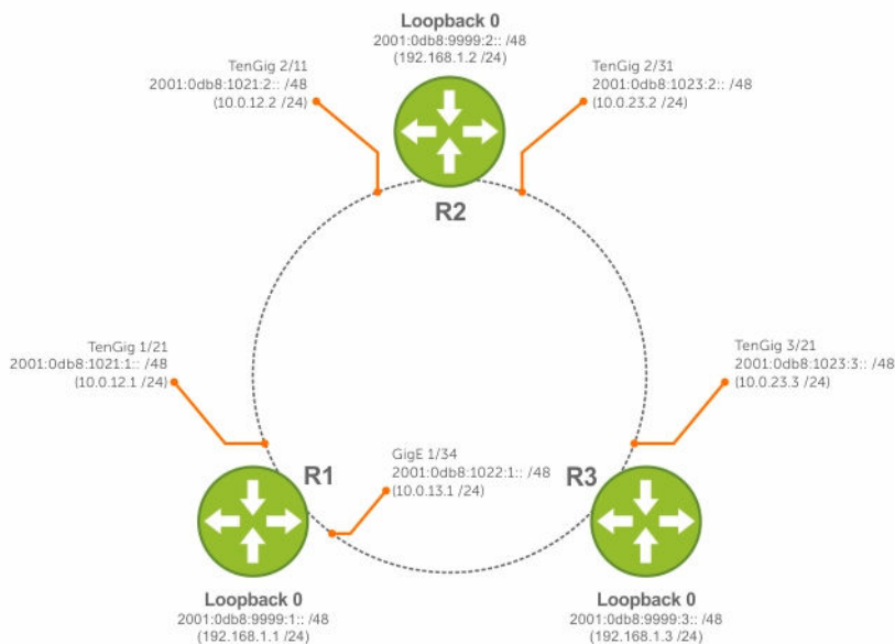
Figure 59. IPv6 IS-IS Sample Topography
