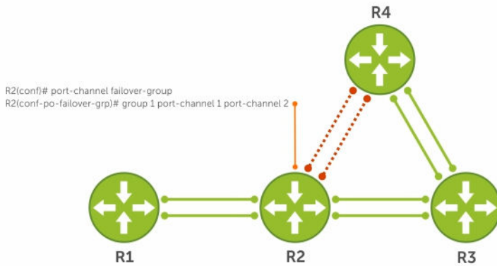
Figure 61. Configuring Shared LAG State Tracking
