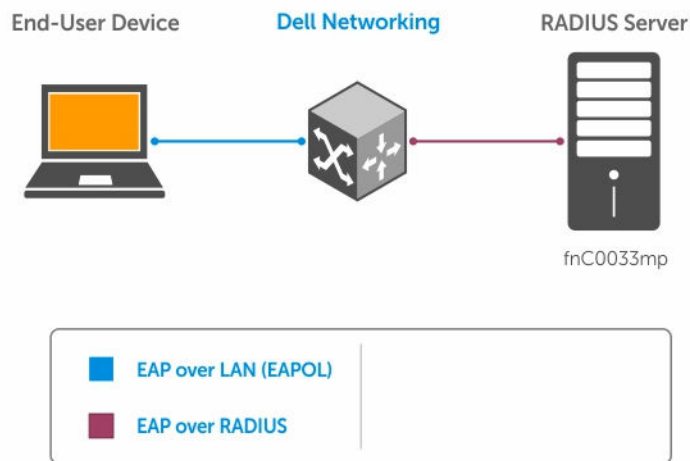
Figure 4. EAP Frames Encapsulated in Ethernet and RADIUS
