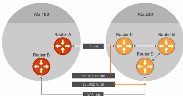
Figure 23. Multi-Exit Discriminators
