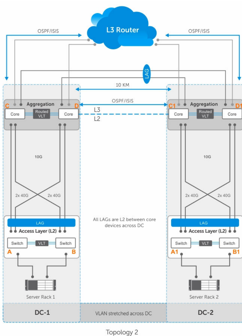
Figure 134. Sample Configuration for a VLT Proxy Gateway
