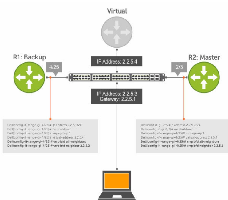
Figure 17. Establishing Sessions with All VRRP Neighbors
