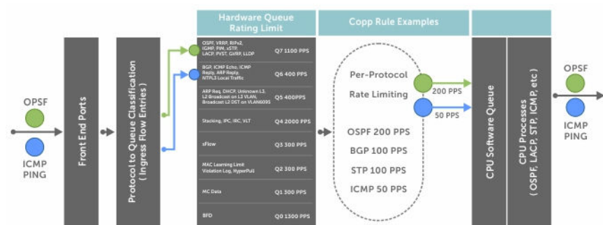
Figure 26. Control Plane Policing
