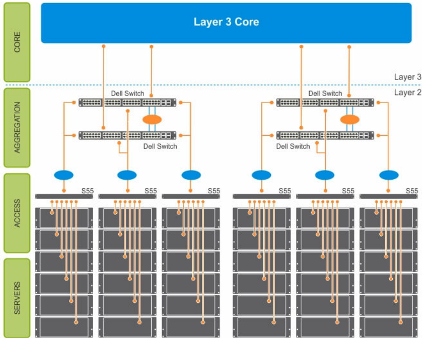
Figure 136. Enhanced VLT
