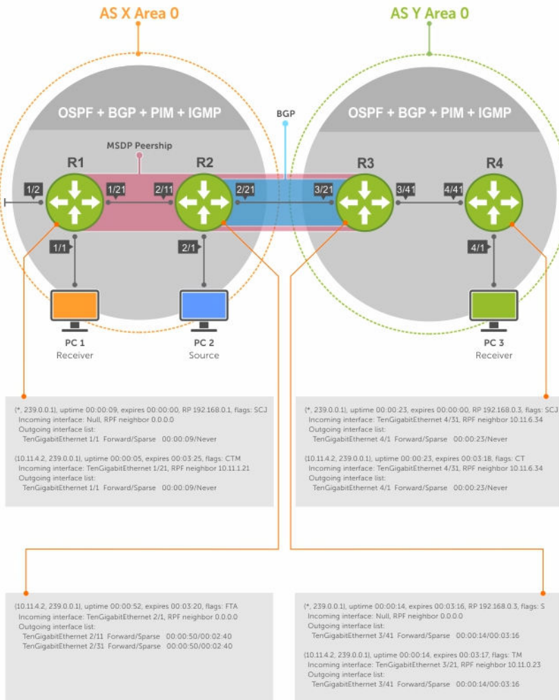
Figure 90. MSDP with Anycast RP
