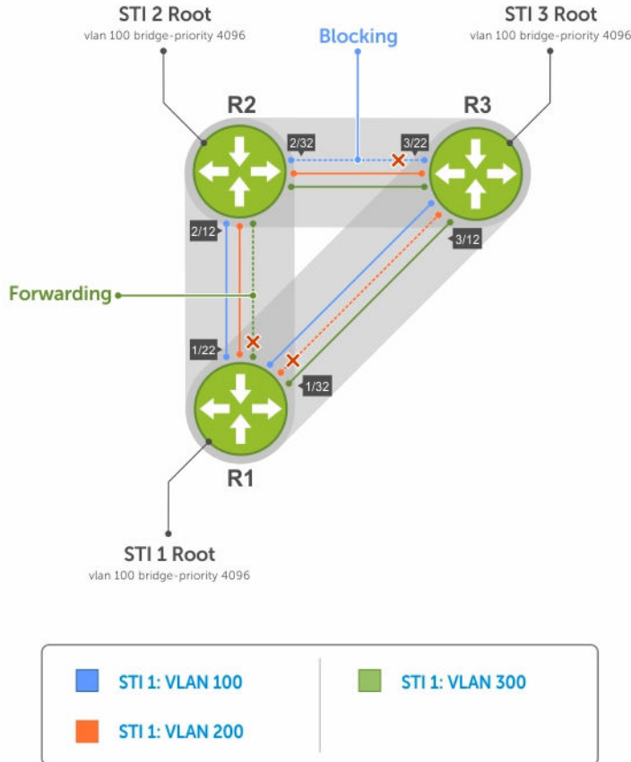
Figure 106. Load Balancing with PVST+
