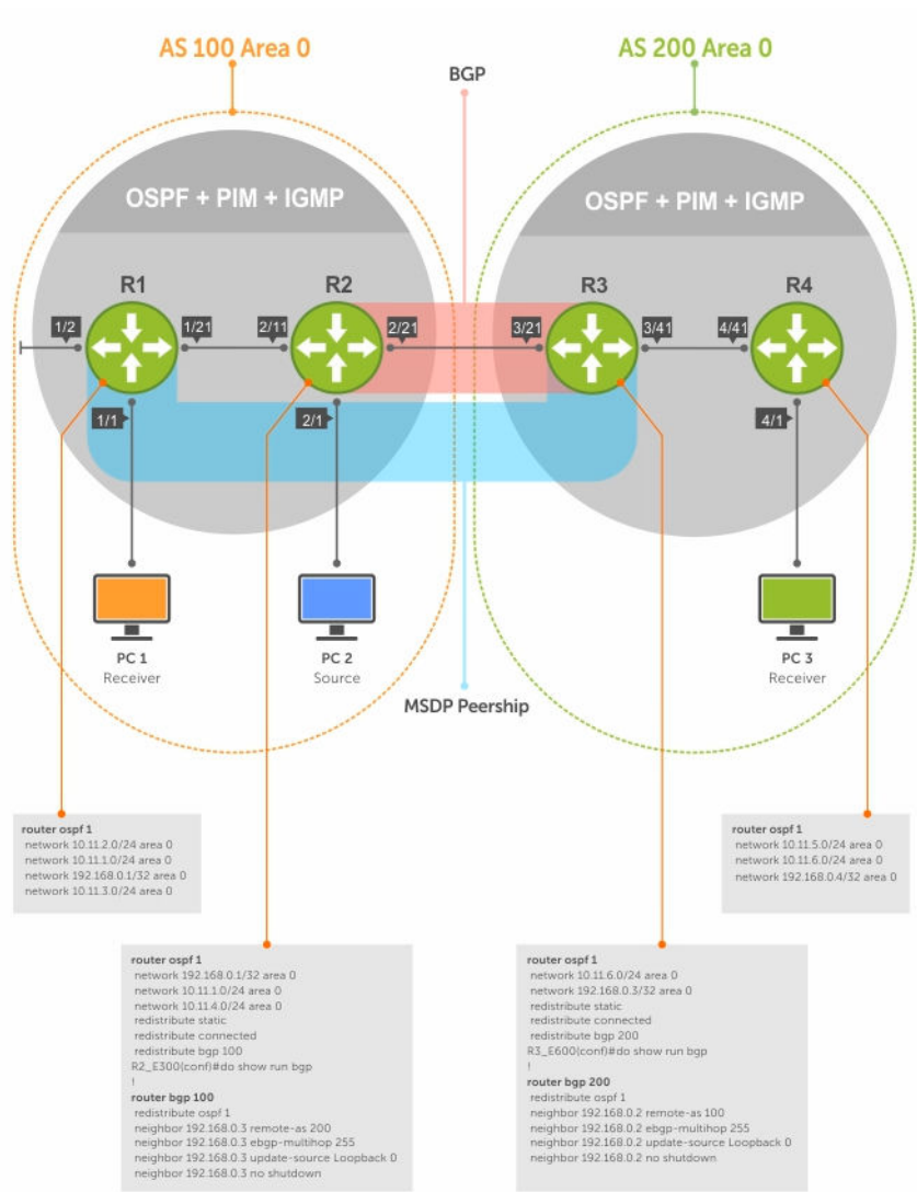
Figure 84. Configuring OSPF and BGP for MSDP
