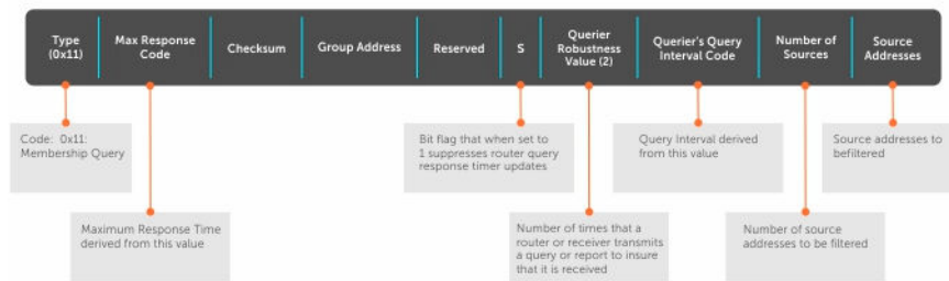
Figure 44. IGMP Version 3 Packet Structure
