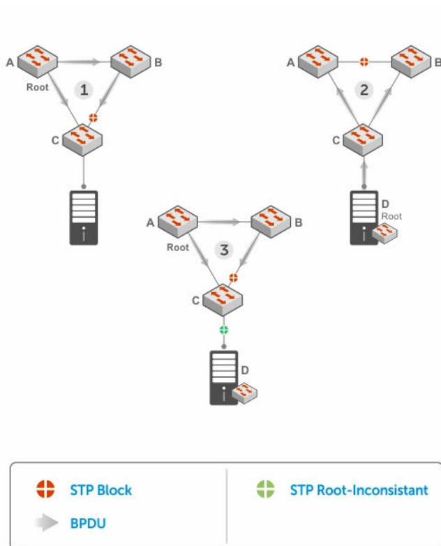
Figure 126. STP Root Guard Prevents Bridging Loops
