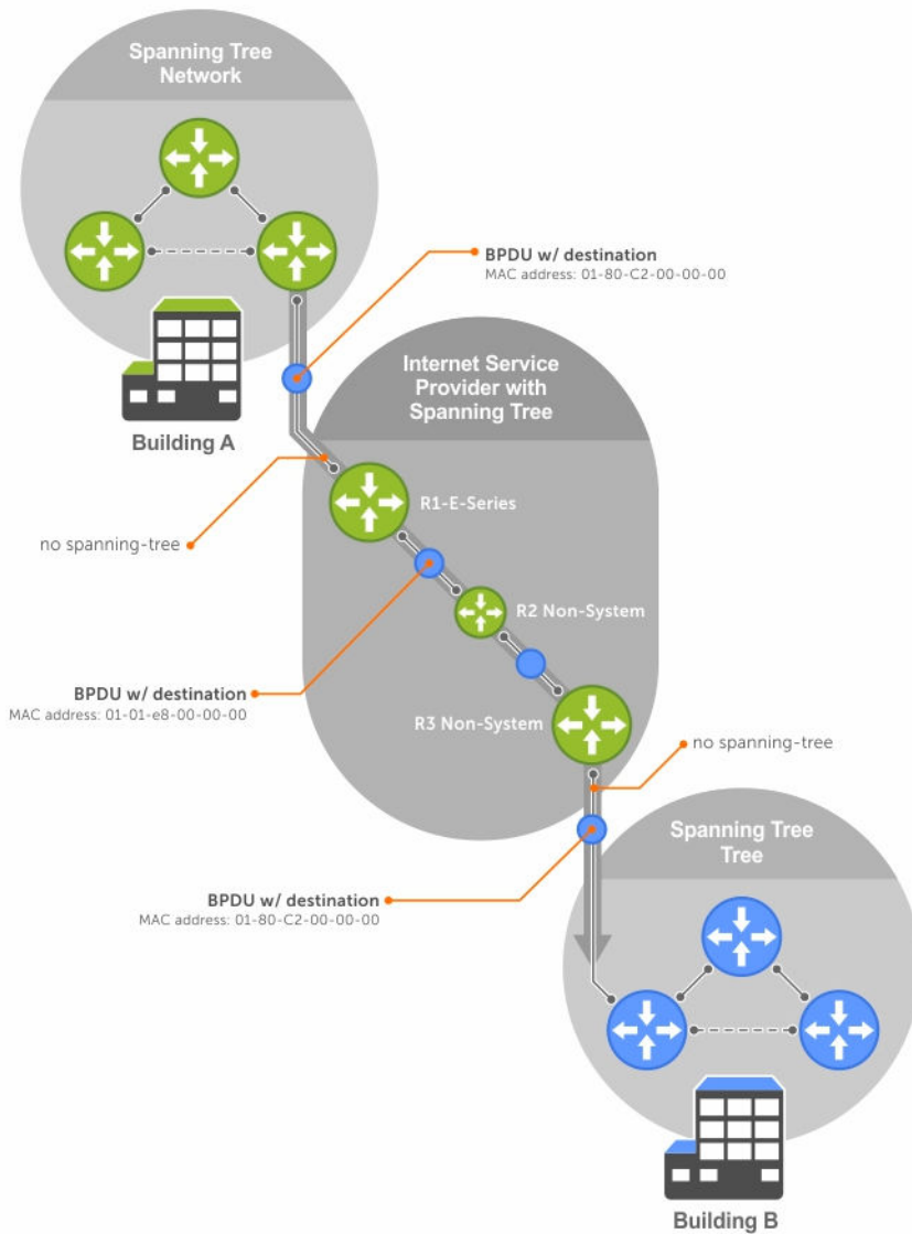
Figure 119. VLAN Stacking with L2PT
