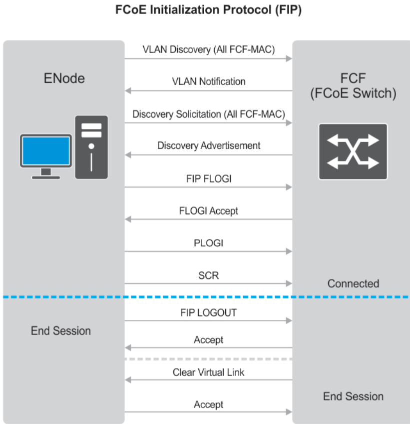
Figure 38. FIP Discovery and Login Between an ENode and an FCF
