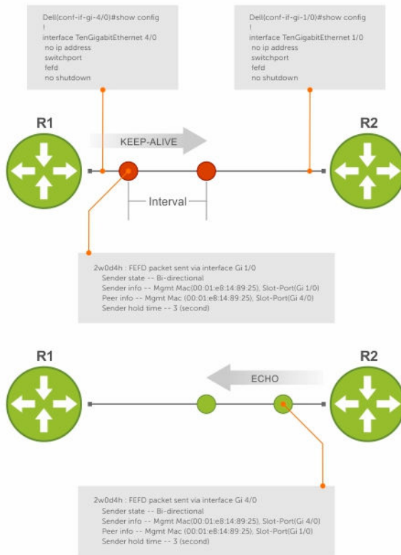
Figure 72. Configuring Far-End Failure Detection
