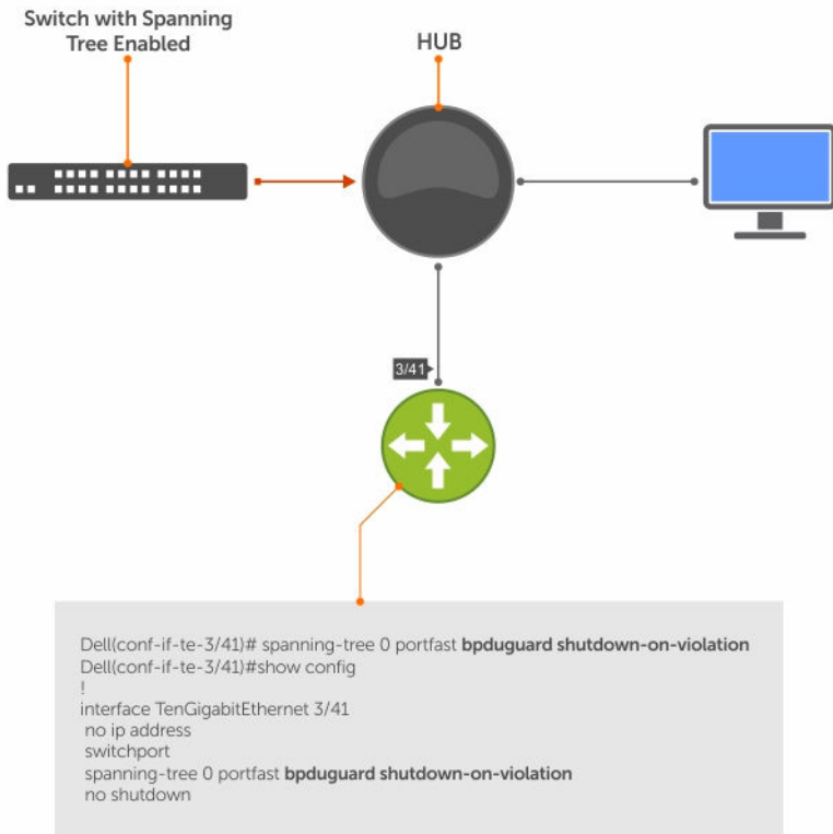
Figure 125. Enabling BPDU Guard
