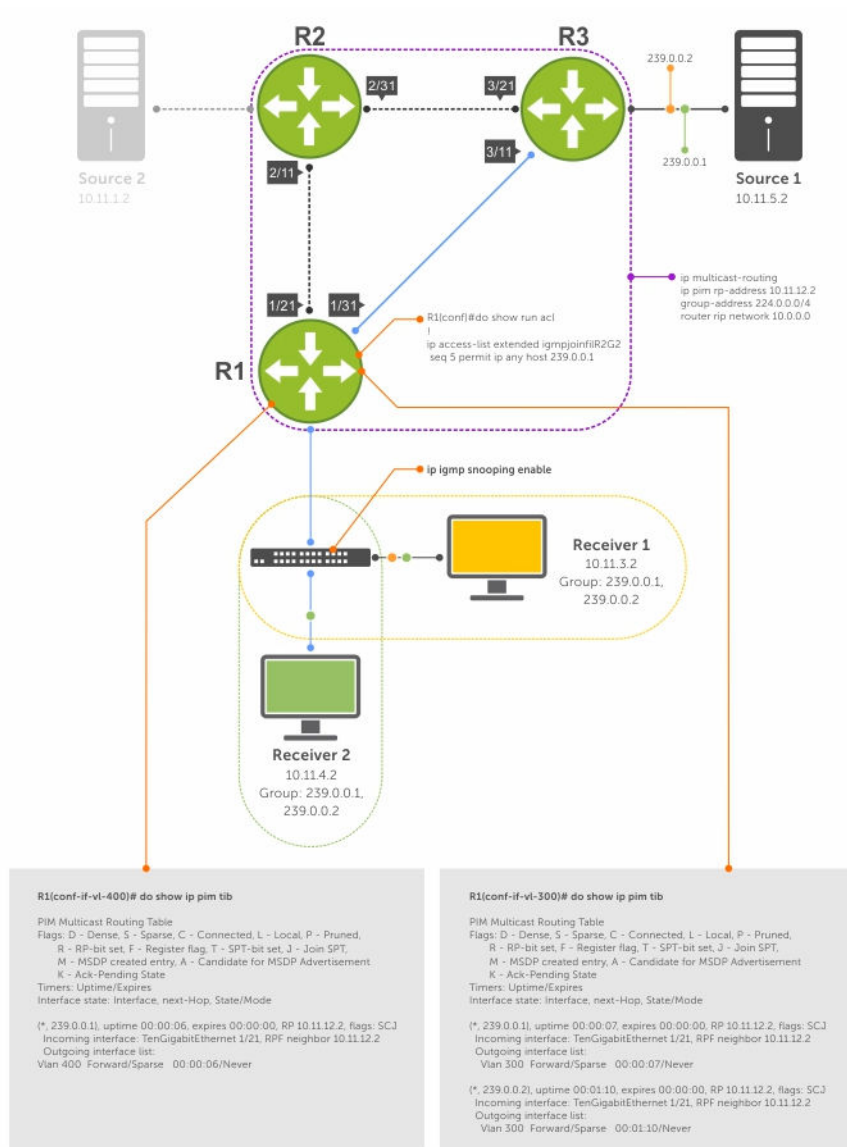
Figure 48. Preventing a Host from Joining a Group
