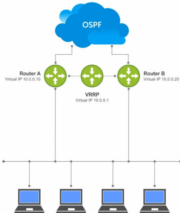
Figure 95. Object Tracking Example
