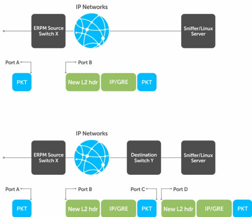
Figure 103. ERPM Behavior
