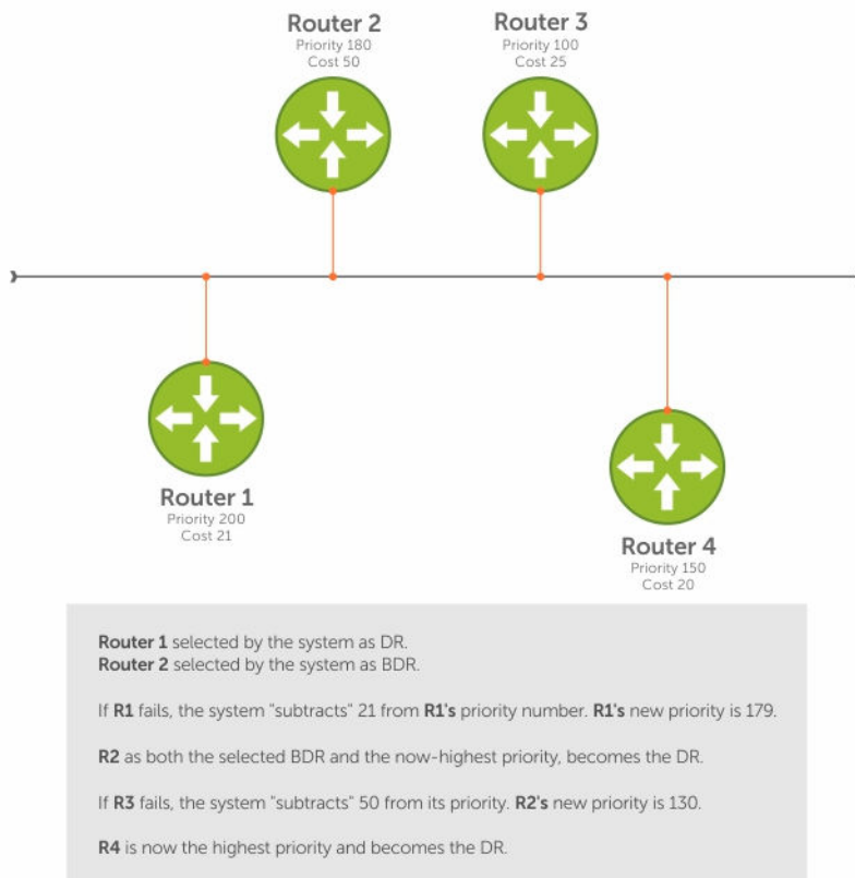
Figure 98. Priority and Cost Examples
