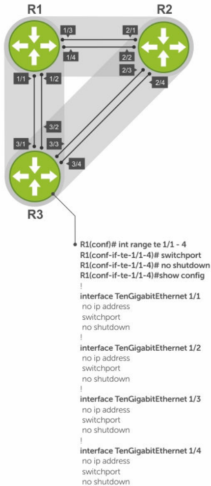
Figure 123. Example of Configuring Interfaces for Layer 2 Mode
