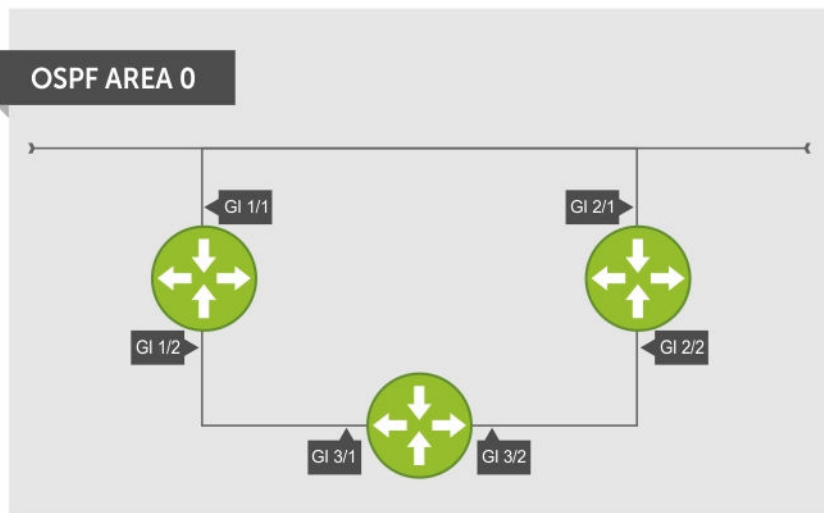
Figure 99. Basic Topology and CLI Commands for OSPFv2
