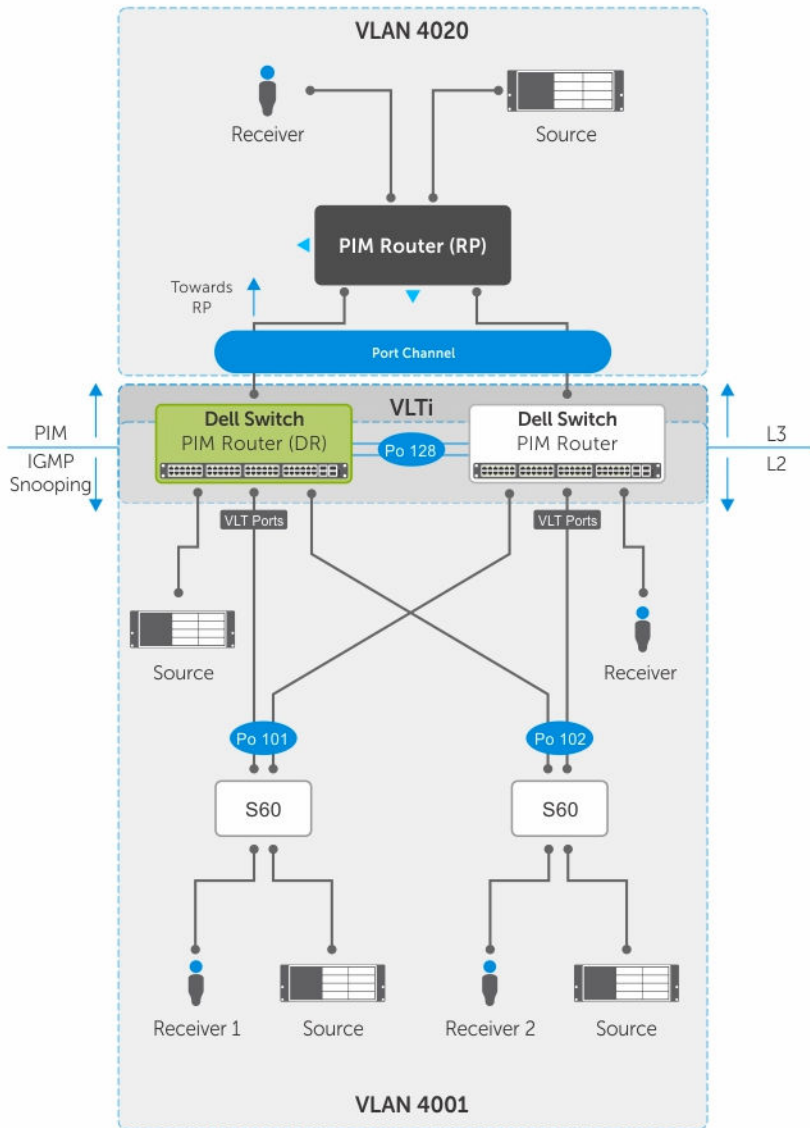
Figure 137. PIM-Sparse Mode Support on VLT
