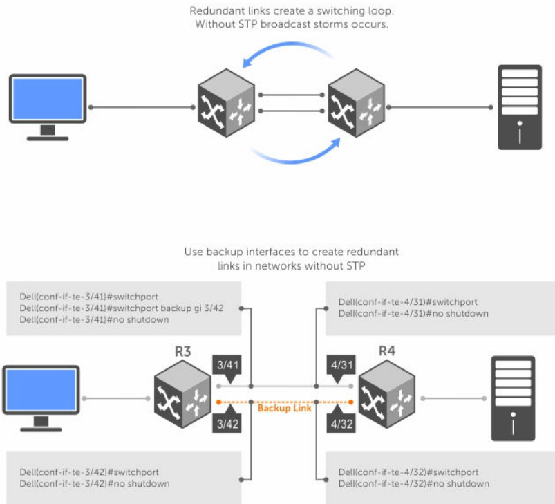
Figure 71. Configuring Redundant Layer 2 Pairs without Spanning Tree
