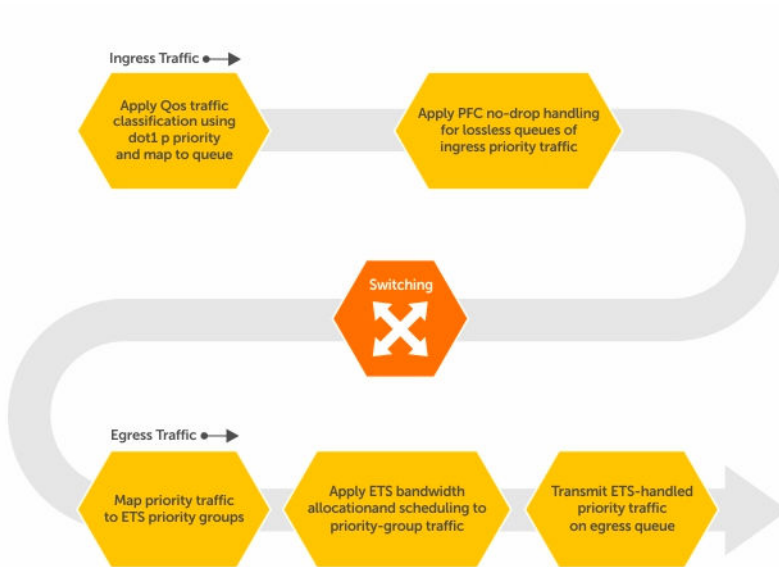
Figure 30. DCB PFC and ETS Traffic Handling
