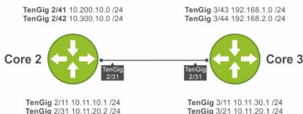
Figure 111. RIP Topology Example
