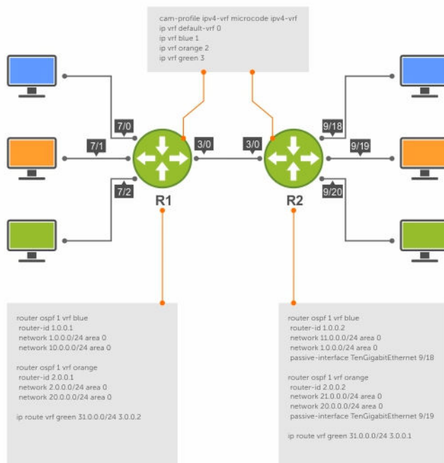
Figure 151. Setup OSPF and Static Routes
