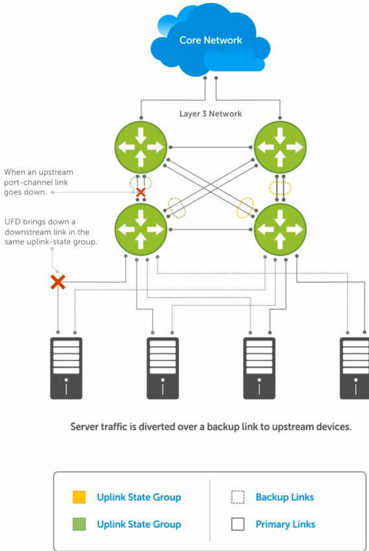
Figure 130. Uplink Failure Detection
