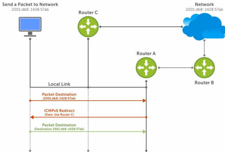
Figure 56. NDP Router Redirect
