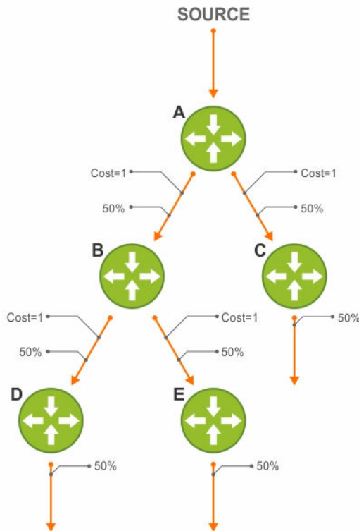
Figure 36. Before Polarization Effect
