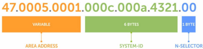
Figure 58. ISO Address Format
