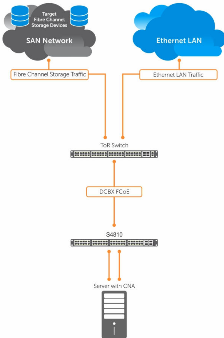
Figure 39. FIP Snooping on a Dell Networking Switch
