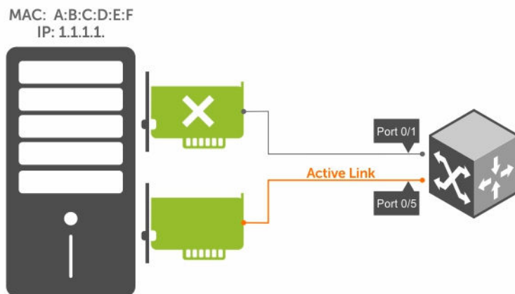
Figure 69. Redundant NICs with NIC Teaming
