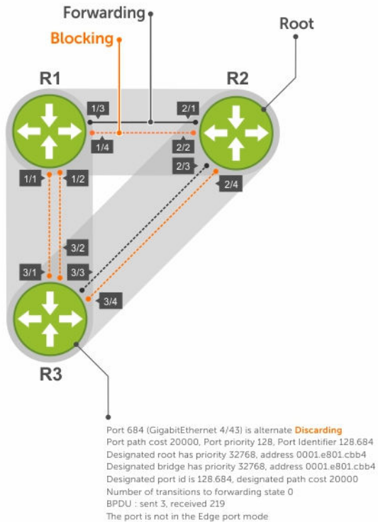
Figure 112. Rapid Spanning Tree Enabled Globally
