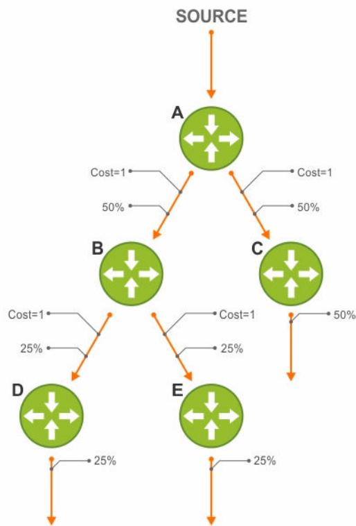
Figure 37. After Polarization Effect
