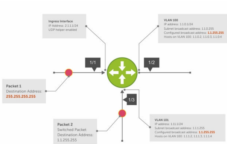
Figure 53. UDP Helper with Configured Broadcast Addresses
