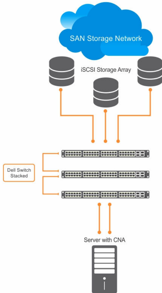
Figure 57. iSCSI Optimization Example
