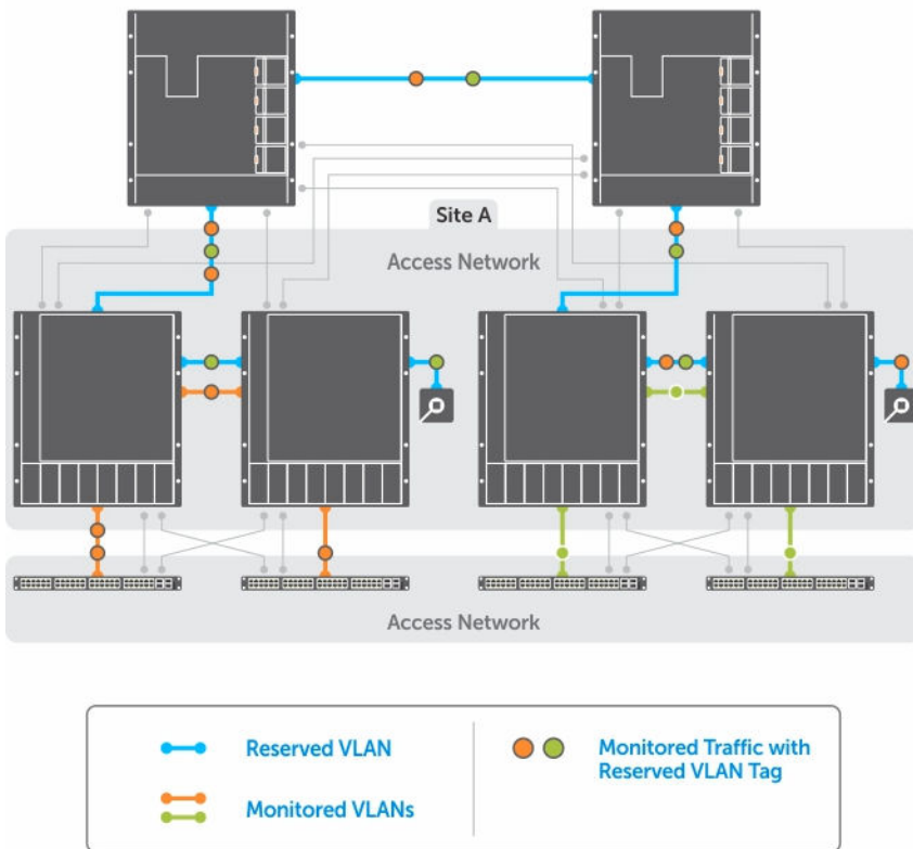
Figure 102. Remote Port Mirroring
