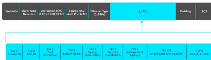
Figure 74. LLDPDU Frame
