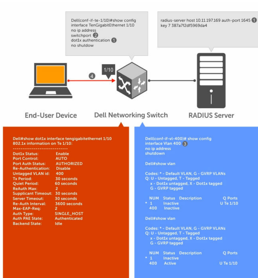
Figure 8. Dynamic VLAN Assignment
