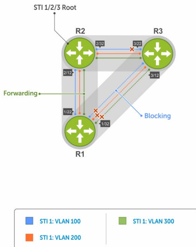
Figure 105. Per-VLAN Spanning Tree
