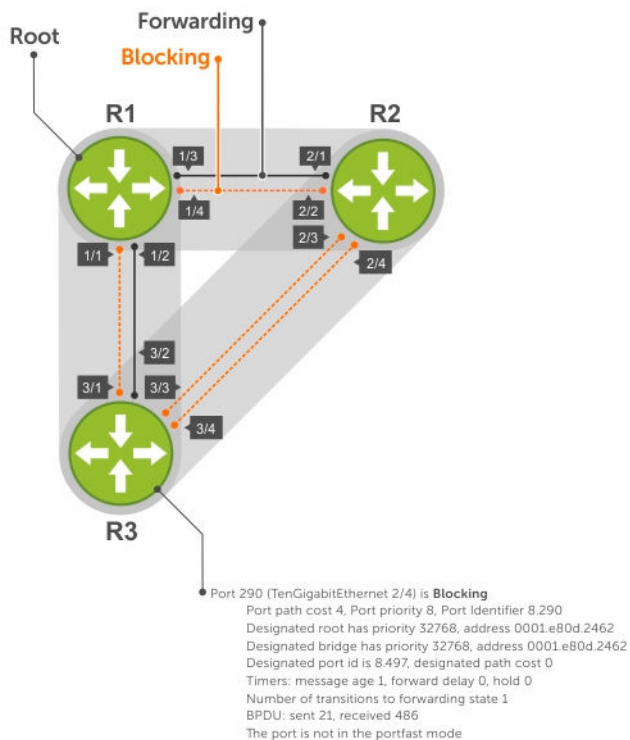
Figure 124. Spanning Tree Enabled Globally
