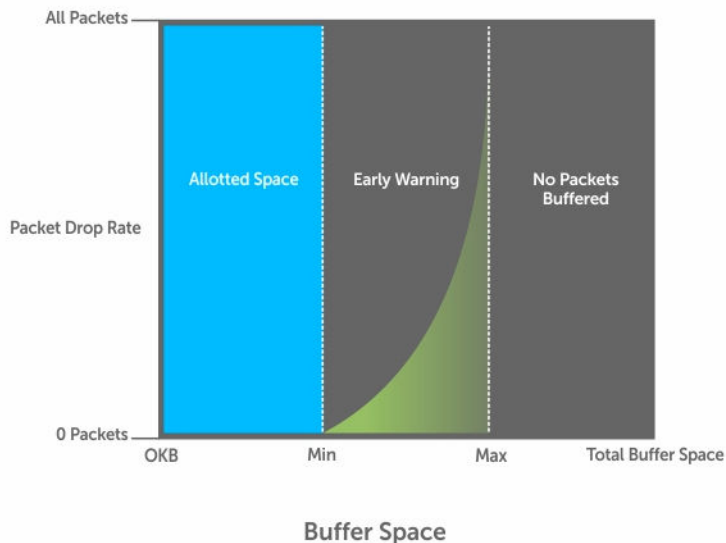
Figure 110. Packet Drop Rate for WRED
