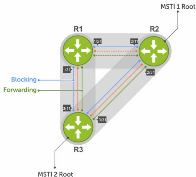
Figure 91. MSTP with Three VLANs Mapped to TWO Spanning Tree Instances
