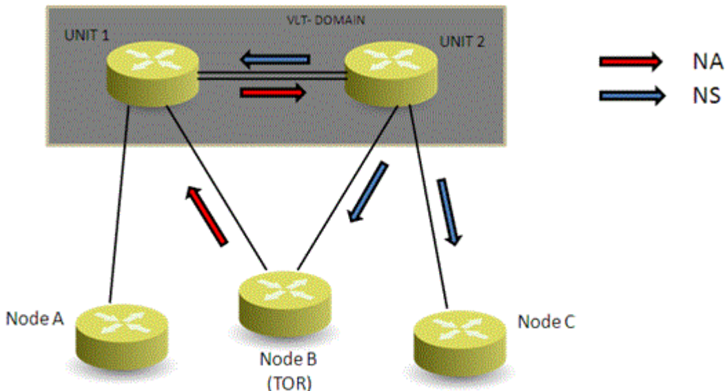
Figure 139. Sample Configuration of IPv6 Peer Routing in a VLT Domain
