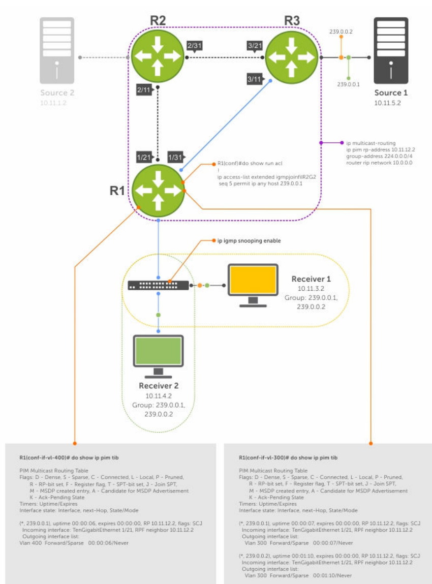
Figure 93. Preventing a Host from Joining a Group
