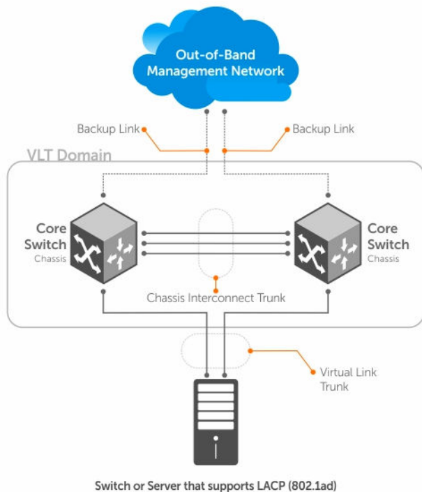
Figure 135. Example of VLT Deployment
