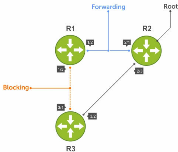
Figure 92. MSTP with Three VLANs Mapped to Two Spanning Tree Instances
