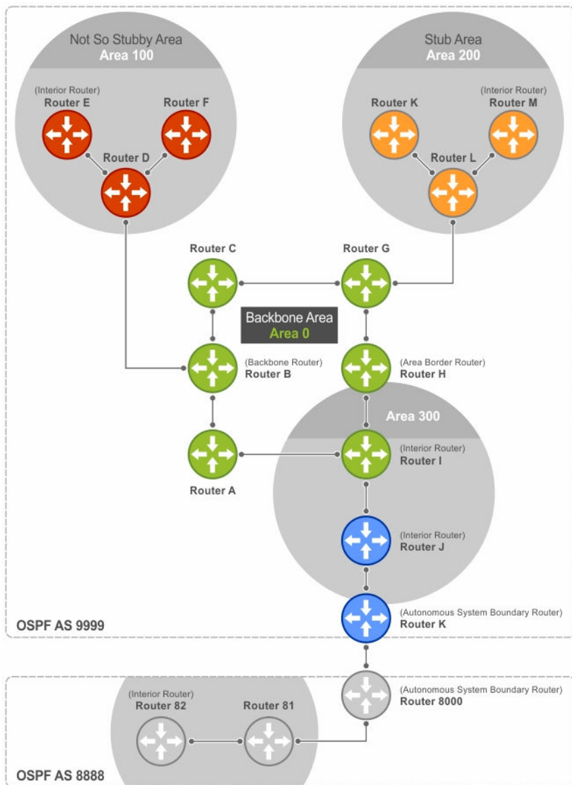
Figure 97. OSPF Routing Examples
