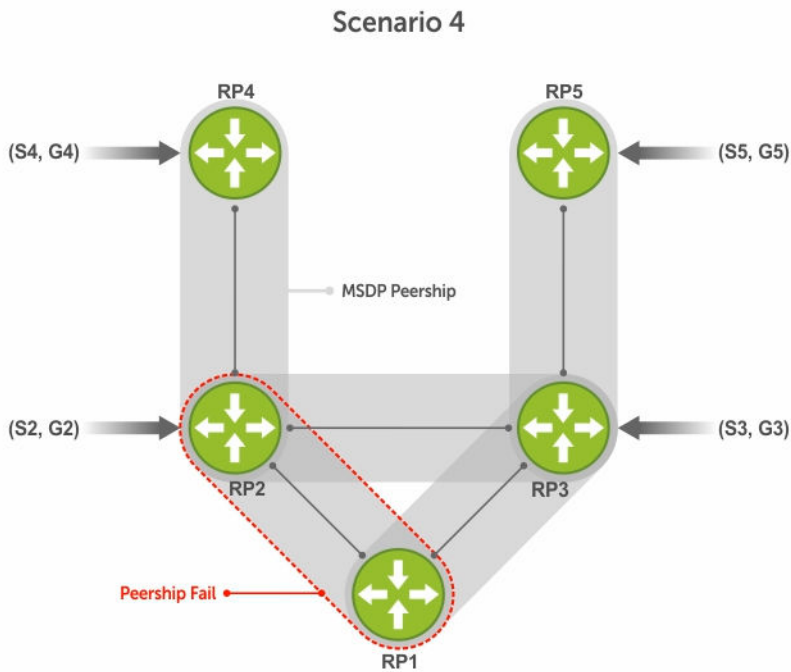
Figure 89. MSDP Default Peer, Scenario 4
