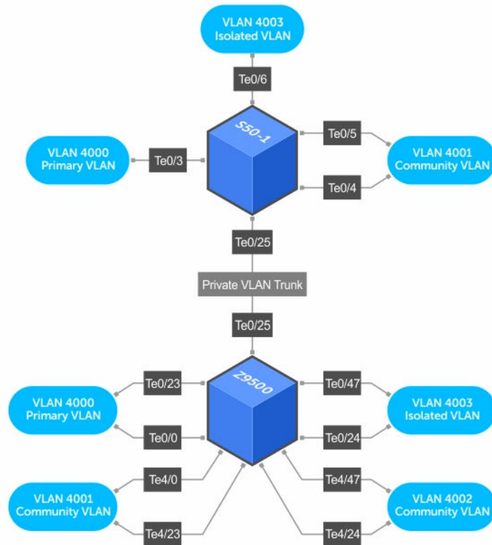
Figure 104. Sample Private VLAN Topology
