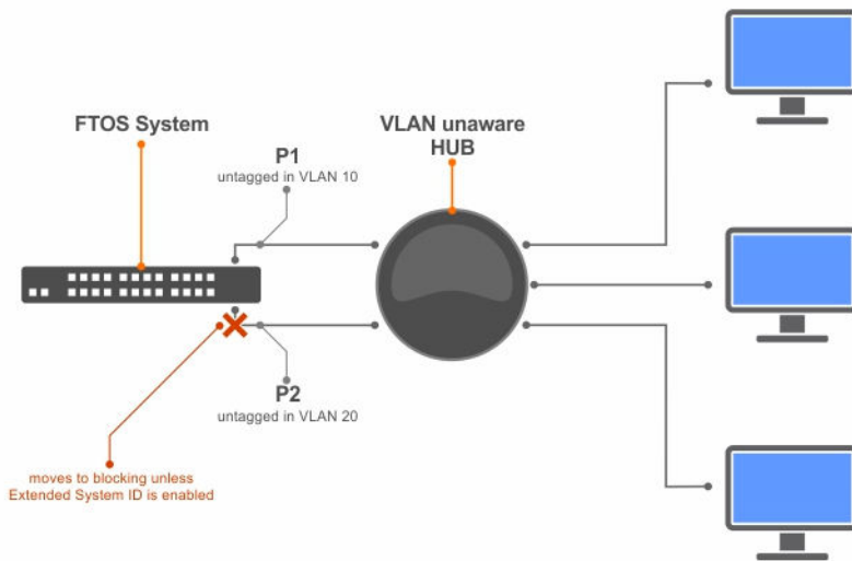
Figure 107. PVST+ with Extend System ID
