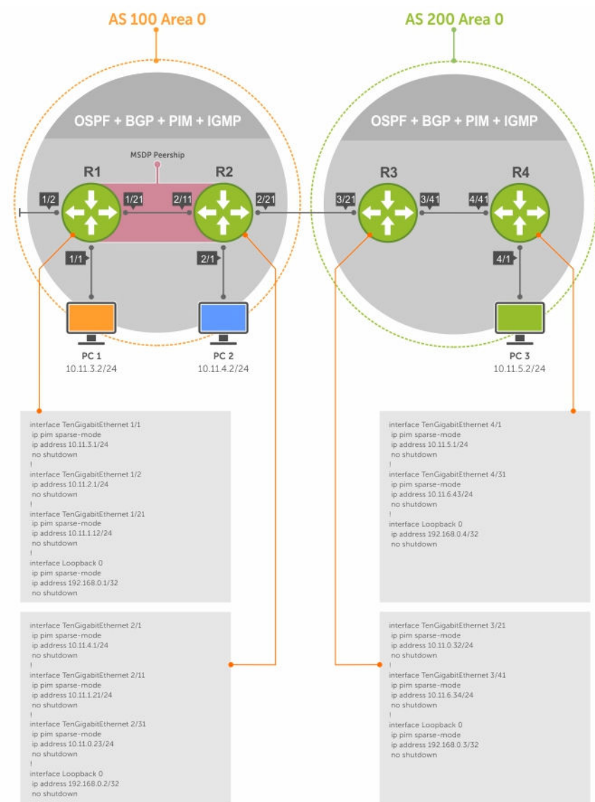
Figure 86. Configuring MSDP
