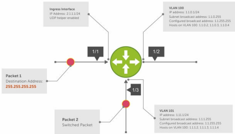
Figure 51. UDP Helper with Broadcast-All Addresses
