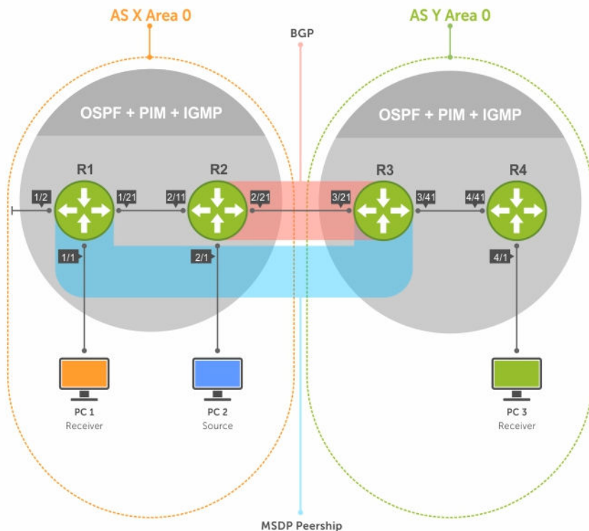
Figure 81. Multicast Source Discovery Protocol (MSDP)
